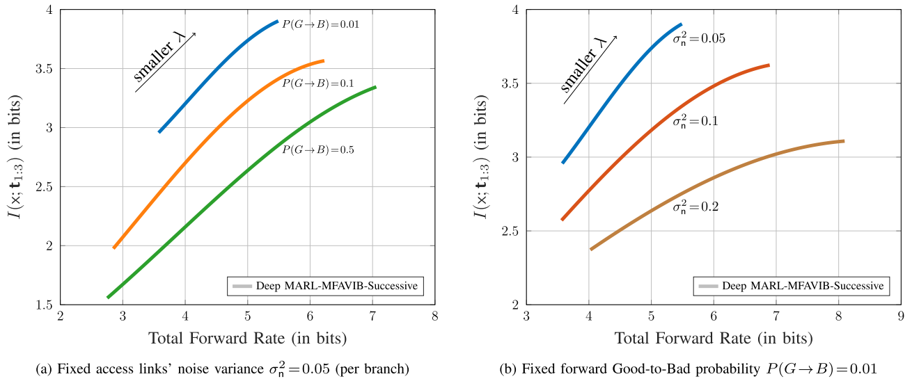
FIGURE 5. The relevant information I(x; \mathbf{t}_{1:3}) vs. total forward rate \sum_j I(y_j; \mathbf{z}_j | \mathbf{t}_{1:j-1}) for a) fixed access noise variance, and b) fixed forward Good-to-Bad transition probability. Equiprobable (power-normalized) 16-QAM source signaling over AWGN access channels and Gilbert-Elliott forward channels. These results have been obtained for fixed output cardinality N=16 by varying the common trade-off parameter 0 \leq \lambda \leq 0.2 for both a) & b).
