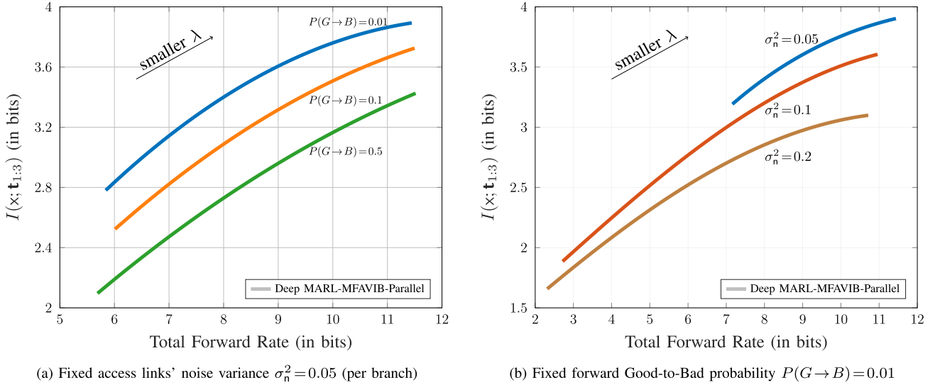
FIGURE 4. The relevant information I(x; \mathbf{t}_{1:3}) vs. total forward rate \sum_j I(y_j; \mathbf{z}_j) for a) fixed access noise variance, and b) fixed forward Good-to-Bad transition probability. Equiprobable (power-normalized) 16-QAM source signaling over AWGN access channels and Gilbert-Elliott forward channels. These results have been obtained for fixed output cardinality N=16 by varying the common trade-off parameter a) 0 \leq \lambda \leq 1 and b) 0 \leq \lambda \leq 0.4 .
