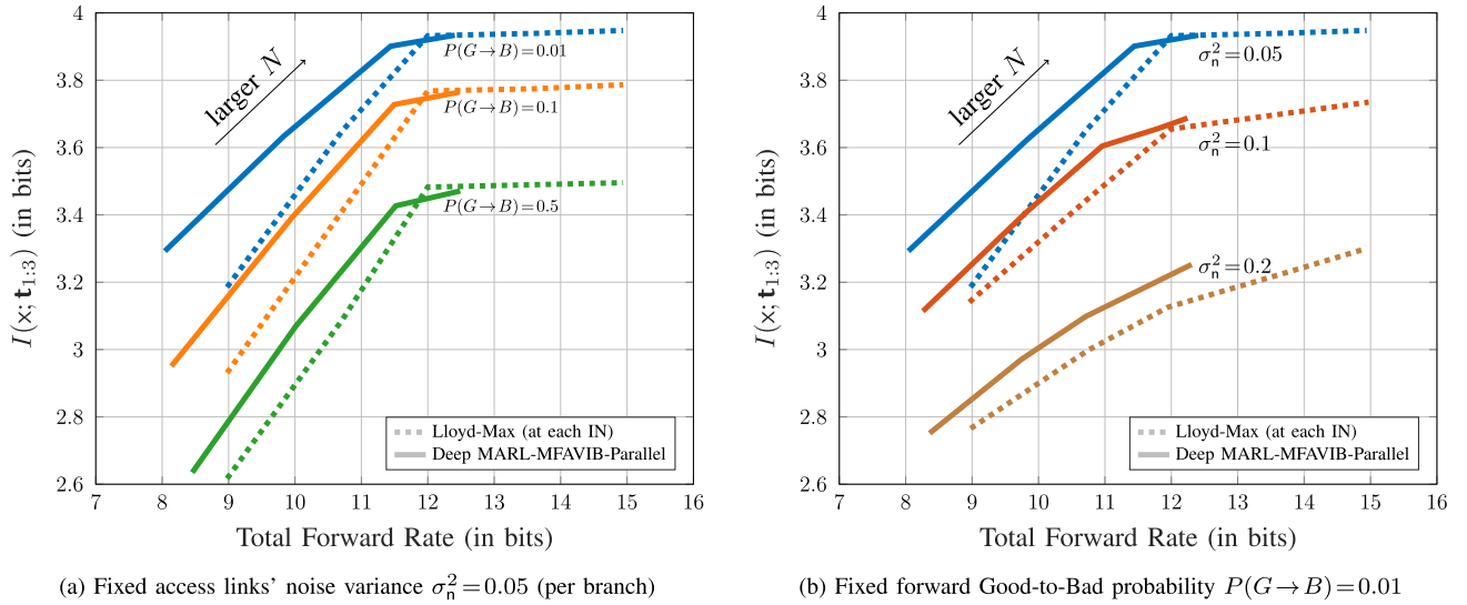
FIGURE 3. The relevant information I(x; t_{1:3}) vs. total forward rate \sum_j I(y_j; z_j) for a) fixed access noise variance, and b) fixed forward Good-to-Bad transition probability. Equiprobable (power-normalized) 16-QAM source signaling over AWGN access channels and Gilbert-Elliott forward channels. These results have been obtained for fixed common trade-off \lambda = 0 by varying the encoders' output cardinality 8 \leq N \leq 32 (per branch) for both a) & b).
